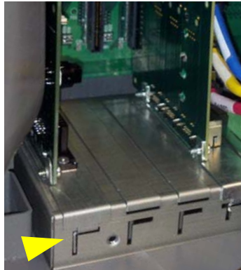
Figure 6. Comm Module Bracket Keyed Slot
