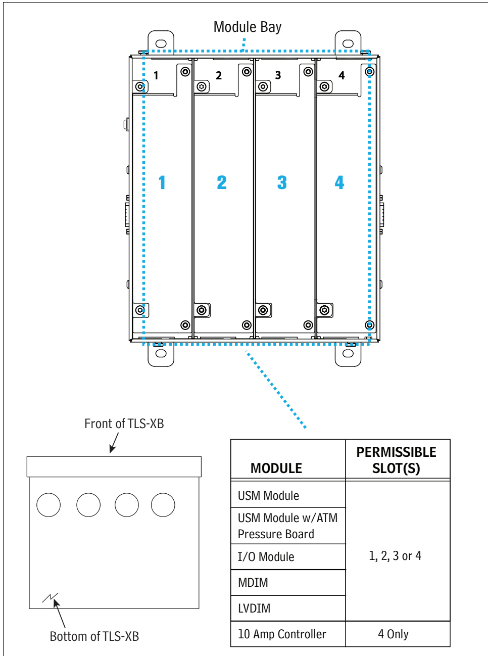
Figure 1. TLS-XB Expansion Box - Plug-in Module Slots (Cover Removed)
