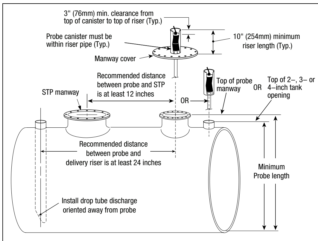
Figure 4. Determining The Minimum Mag Probe Length
