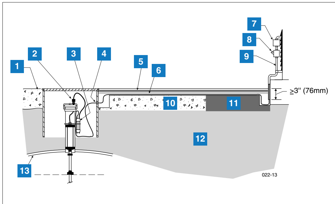
Figure 9. Example Probe Wiring Run via Direct Burial Cable
