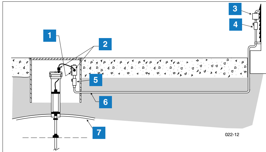
Figure 8. Example Probe Wiring Run in Buried Rigid Conduit
