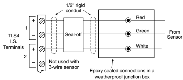
Groundwater Sensor
