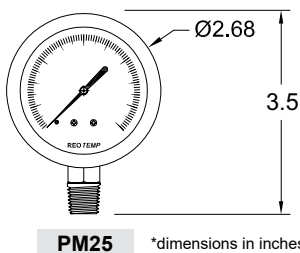
PM25 *dimensions in inches
