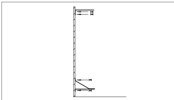
Figure 3 – Installation des supports de montage
