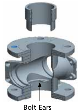
Bolt Ears
