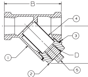
T-221/222-A Threaded
