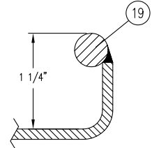
DRUM NECK SECTION SCALE: NONE
