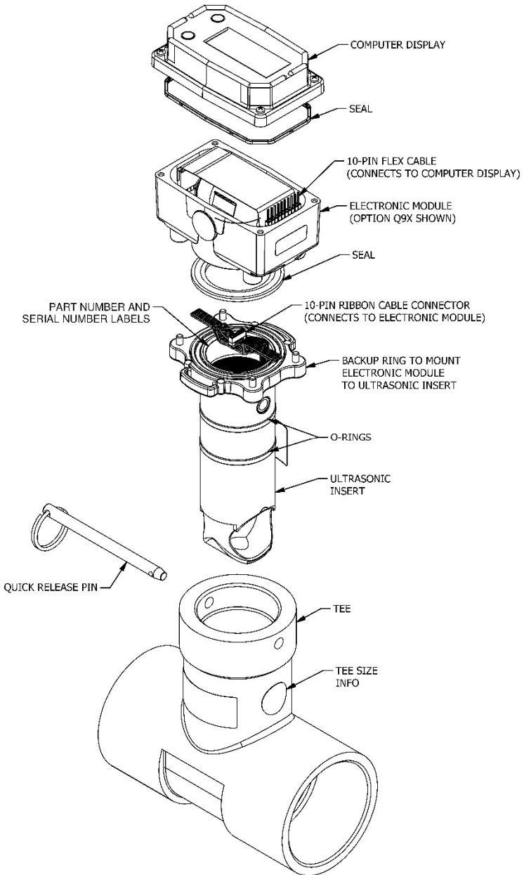
Figure 2 (UM050SK shown)
