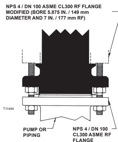
Figure 3. Valve Installation Schematic
