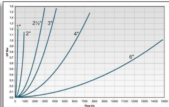
Pressure drop for 1" to 6", scale 0-15000 l/min.
