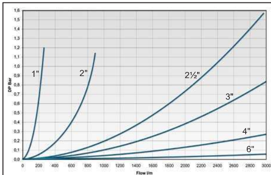
Pressure drop for 1" to 6", scale 0-3000 l/min.
