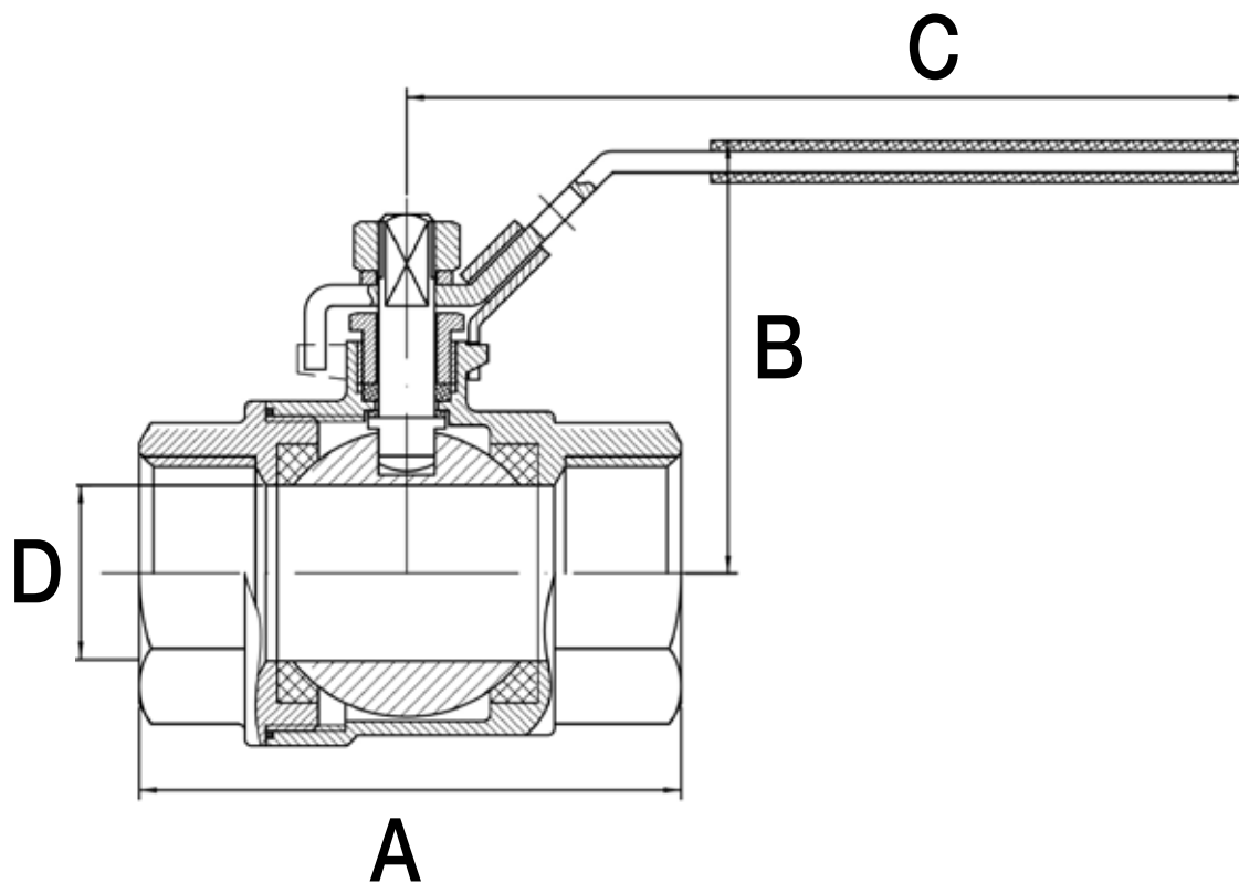
DIMENSIONS (INCHES)
