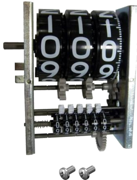
Liter Register and Screws
