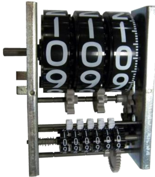
Liter Register (5)
